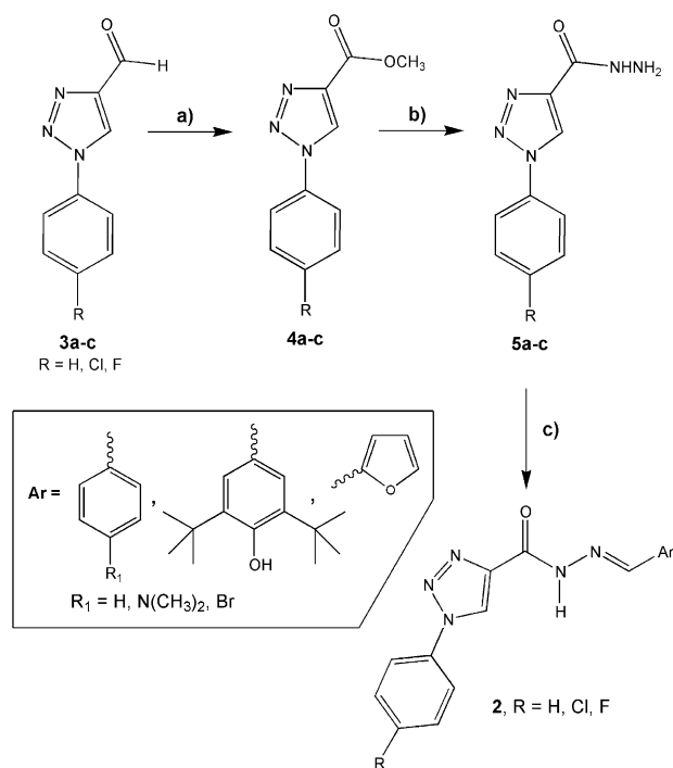
Scheme 1. (a) NaCN, MnO 2 , MeOH, rt, 5–6 h (71–85%); (b) NH 2 NH 2 ·H 2 O 80%, EtOH, reflux, 5–6 h (68–84%); (c) ArCHO, EtOH, HCl (cat.), reflux (32–98%).
