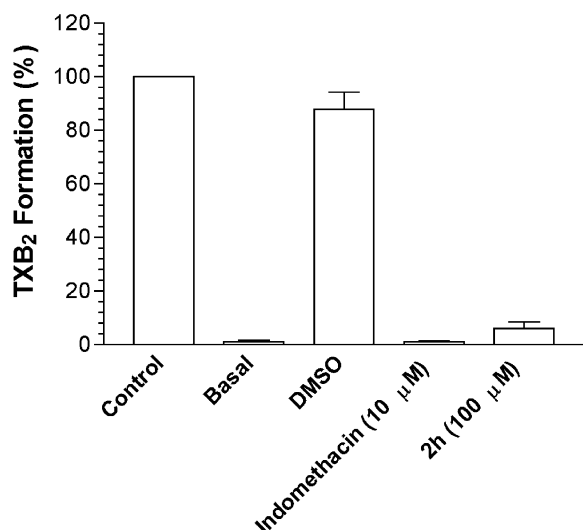
Figure 2. Effects of NAH derivative 2h (100 μM) and indomethacin (10 μM) on platelets TXB 2 formation induced by collagen. Results are expressed as mean ± SEM for n=3 independent experiments. Basal = unstimulated platelets. Control = platelets stimulated by collagen 5 mg/mL. Control was employed as 100% of TXB 2 formation. * p < 0.05 (Student's t -test).
