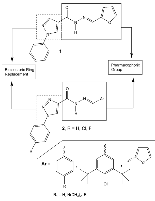
Figure 1. Design concept of N -substituted-phenyl-1,2,3-triazole-4-acylhydrazone derivatives.
